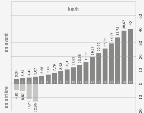
Transmission Full Powershift 19x4 à 40 km/h
